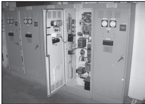
A typical '80s analog exciter control panel crowded with obsolete components
